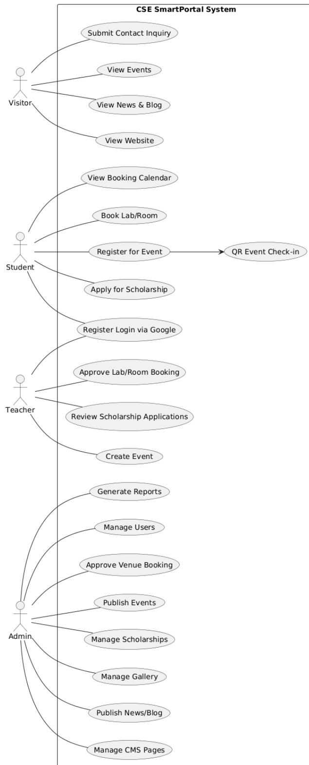
Figure 3.1: Overall System Use Case Diagram for CSE SmartPortal
