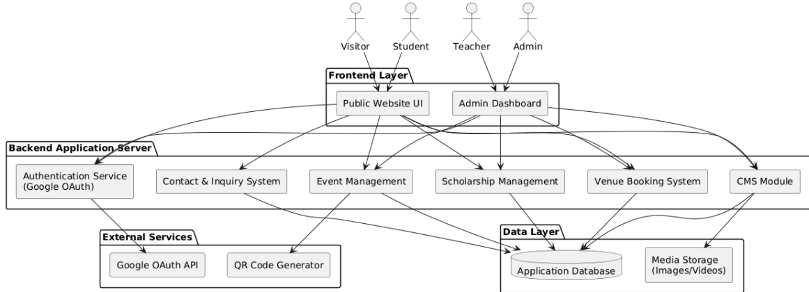
Figure 3.2: System Architecture Diagram for CSE SmartPortal
